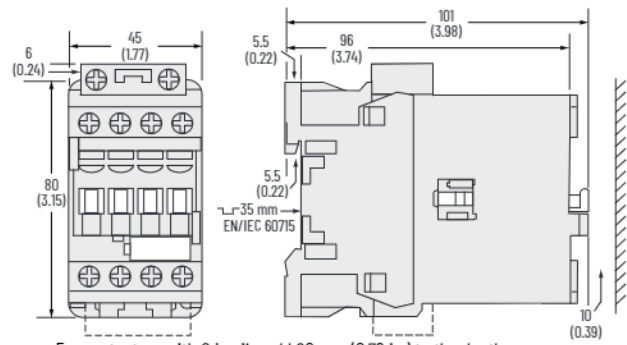
Figure 46 - 100-E26...100-E38 4-Pole Contactors with Low-consumption Coils
